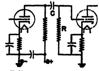
RC coupling in an amplifier.
